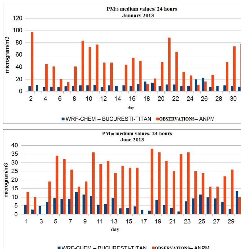
Figure 6. Comparison between medium values/24h of PM 10 concentrations derived from WRF-CHEM model and observational data, at monitoring station București-Titan
