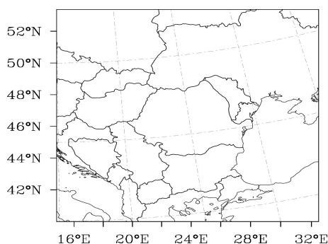
Figure 1. WRF-CHEM integration domain
