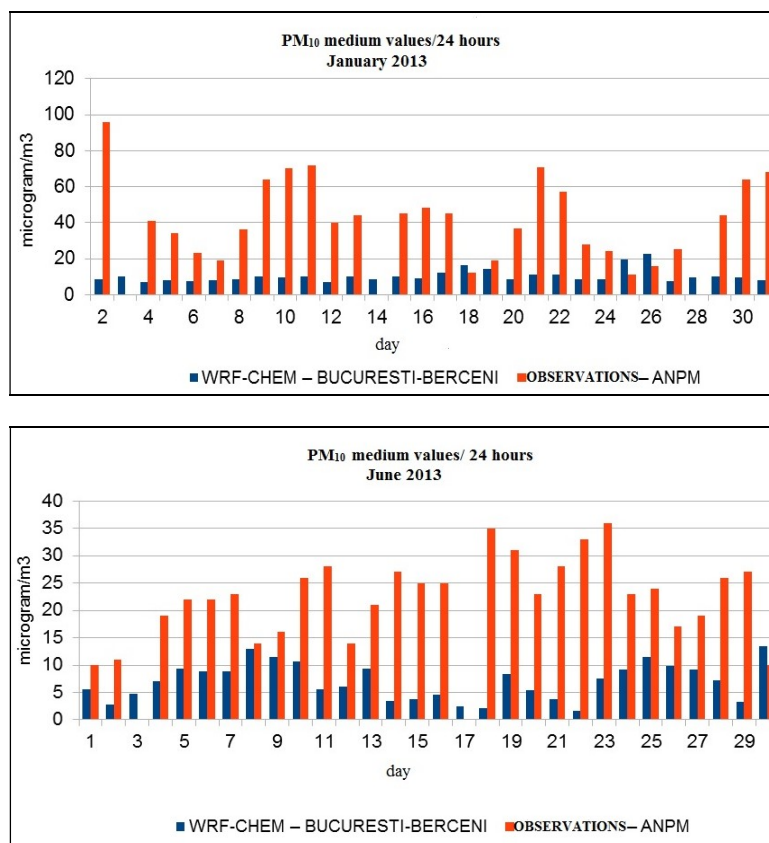
Figure 5. Comparison between medium values/24h of PM_{10} concentrations derived from WRF-CHEM model and observational data, at monitoring station București-Berceni
